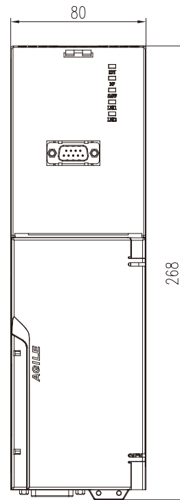
CM25 Control Module's dimensions (Unit:mm)
