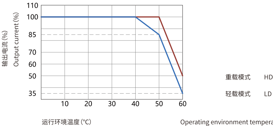
Capacity reduction data & Environment temperature
