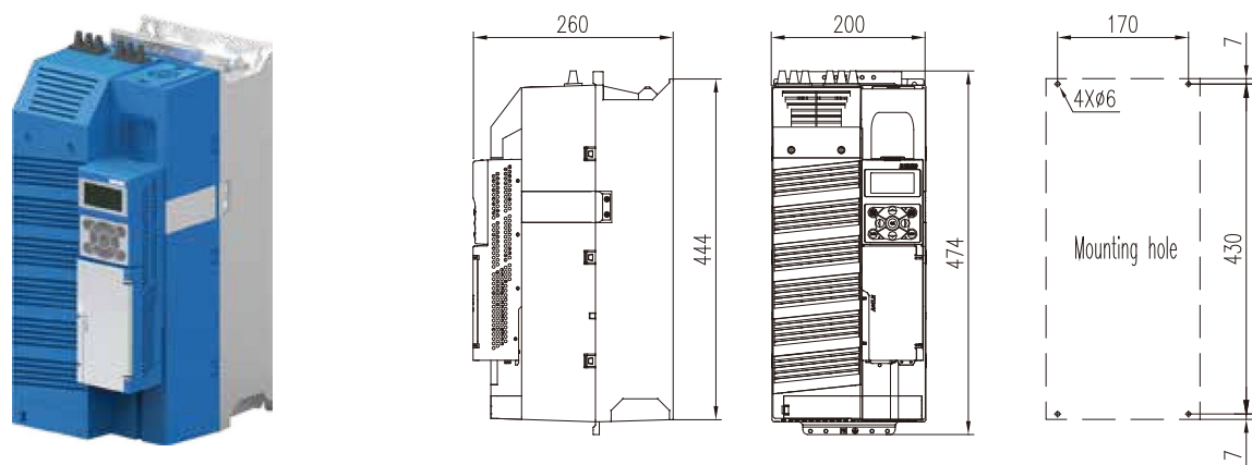
◆B4 (18.5 kW~37kW)
